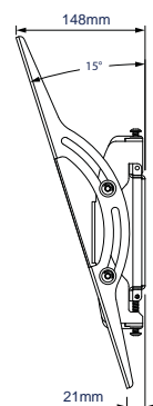
SIDE VIEWS
