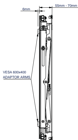
SIDE VIEW CLOSED
