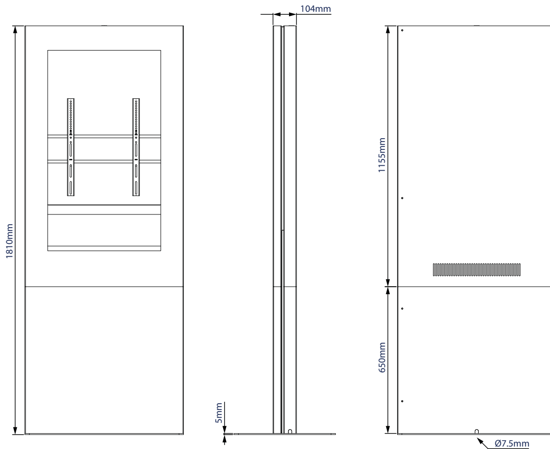
FRONT VIEW
