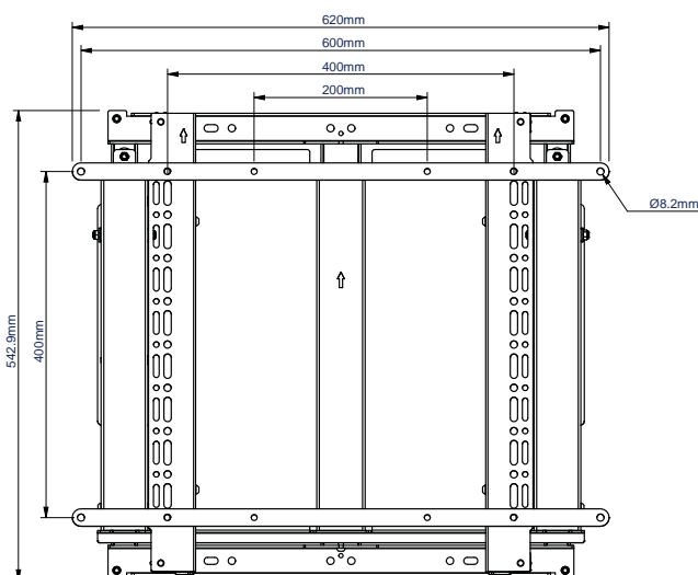
FRONT VIEW WITH ADAPTOR ARMS
