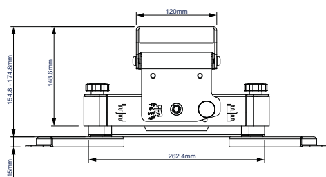
SIDE VIEW WITH EXTENSION LEGS
