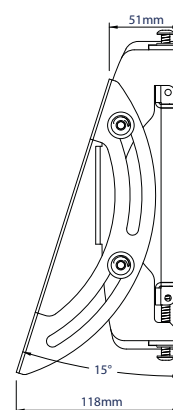
SIDE VIEWS
