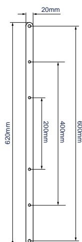
ADAPTOR ARMS
