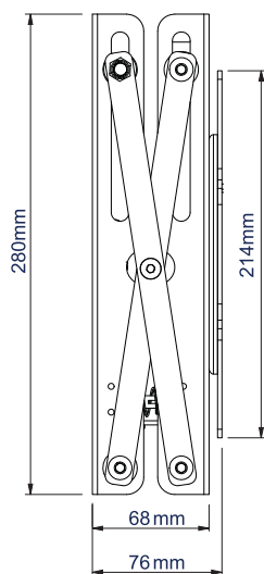
SIDE VIEW CLOSED
