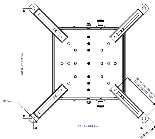
BOTTOM VIEW WITH EXTENSION LEGS
