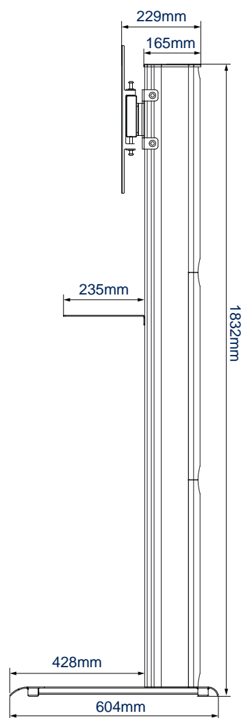
SIDE VIEW
