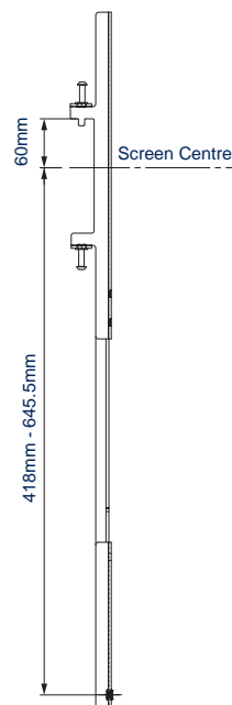
SIDE VIEW MOUNTING BELOW WITH EXTENSION BAR
