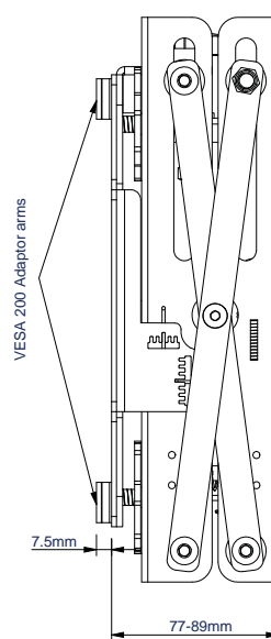
OPEN VIEW EXTENDED
