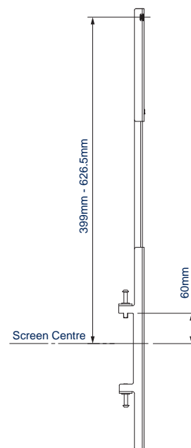
SIDE VIEW MOUNTING ABOVE WITH EXTENSION BAR
