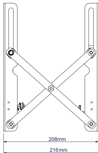
SIDE VIEW EXTENDED
