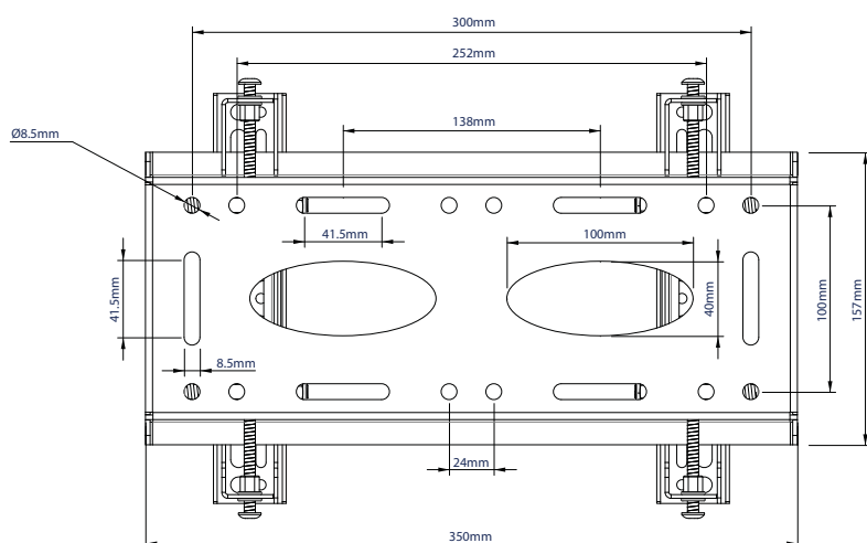
REAR VIEW
