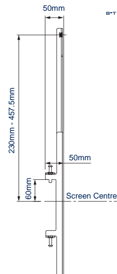
SIDE VIEW MOUNTING ABOVE
