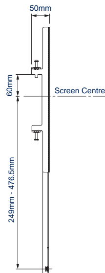
SIDE VIEW MOUNTING BELOW
