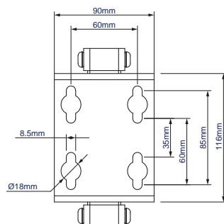
MOUNTING PLATE
